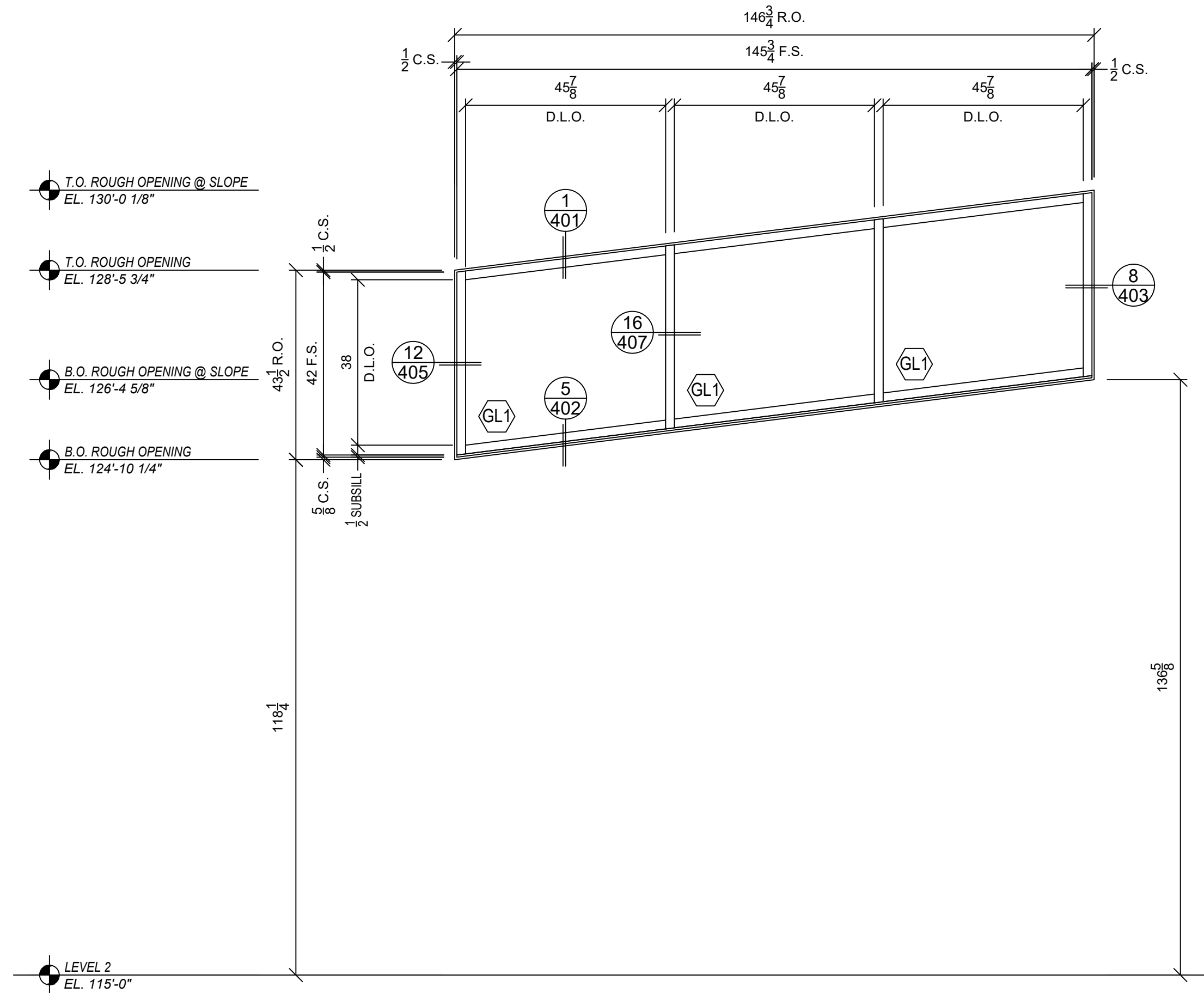
20 ELEVATION SF-12.3 ARCH REF: 2-A4.1.1, 2-A4.2.2 QTY: (1) TUBELITE T24650, 2" X 6.5", OUTSIDE GLAZED
