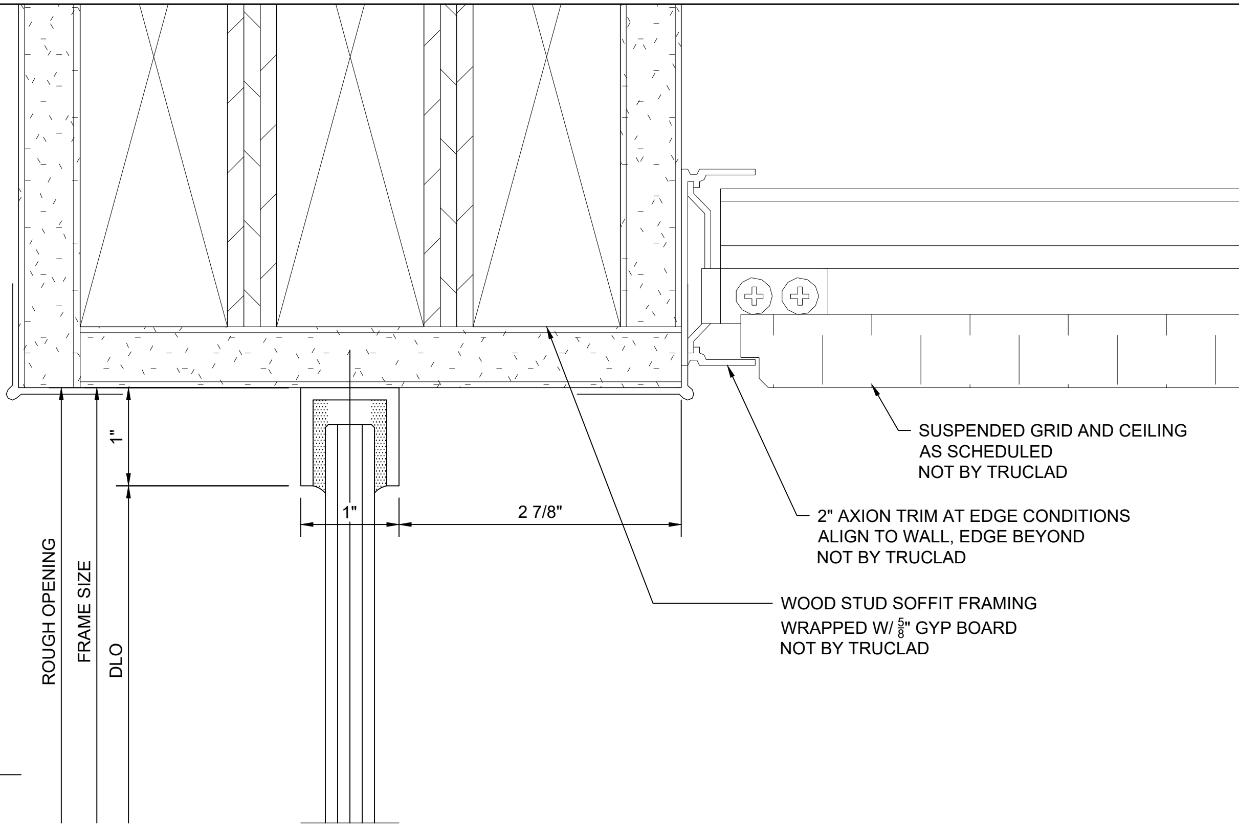
29 STFT-3, SF24 @ BULKHEAD CEILING ARCH REF: 17/2-A7.3.1 1" X 1" GLAZING CHANNEL
