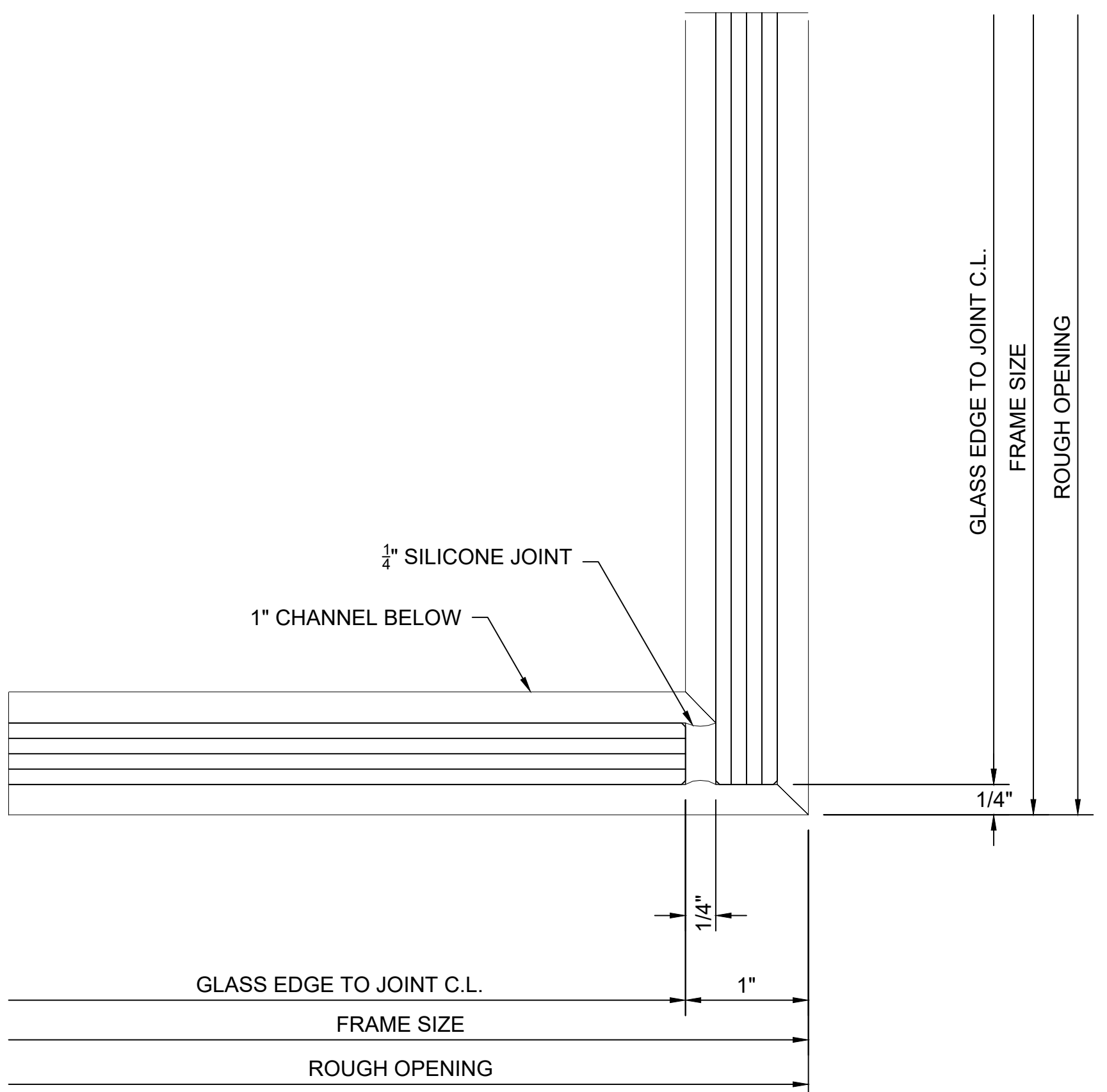
30 STFT-3 CORNER @ SF22/SF23 ARCH REF: 3/2-A4.3.0 1" X 1" GLAZING CHANNEL
