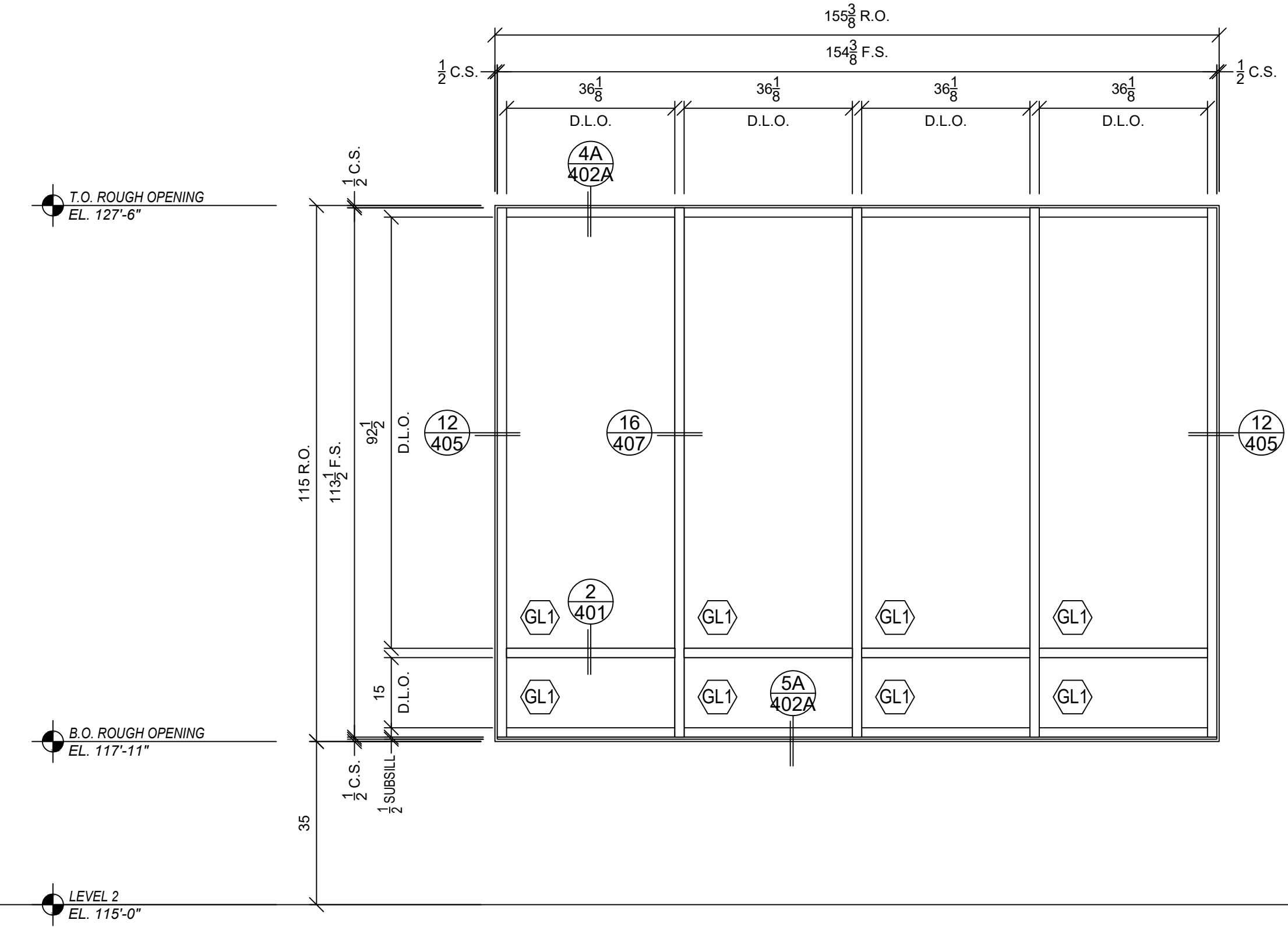
22 ELEVATION SF-13.2 ARCH REF: 2-A4.1.1, 2-A4.2.2 QTY: (1) TUBELITE T24650, 2" X 6.5", OUTSIDE GLAZED
