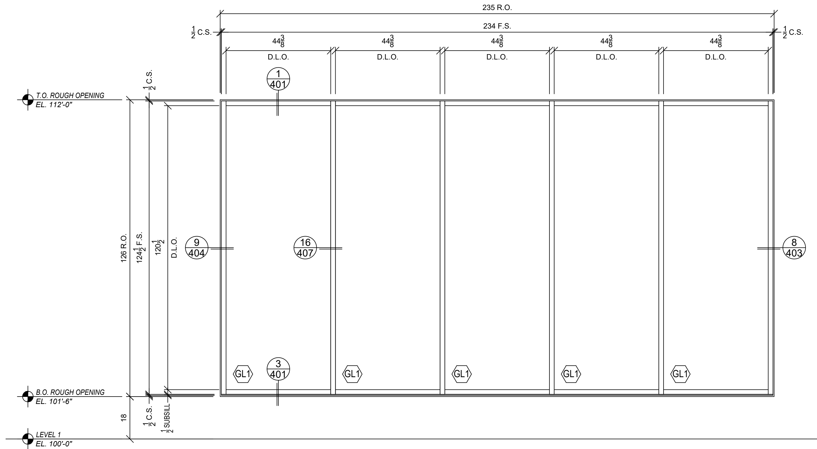
5 ELEVATION SF-3.1 ARCH REF: 2-A4.1.1, 2-A4.2.1 QTY: (1) TUBELITE T24650, 2" X 6.5", OUTSIDE GLAZED
