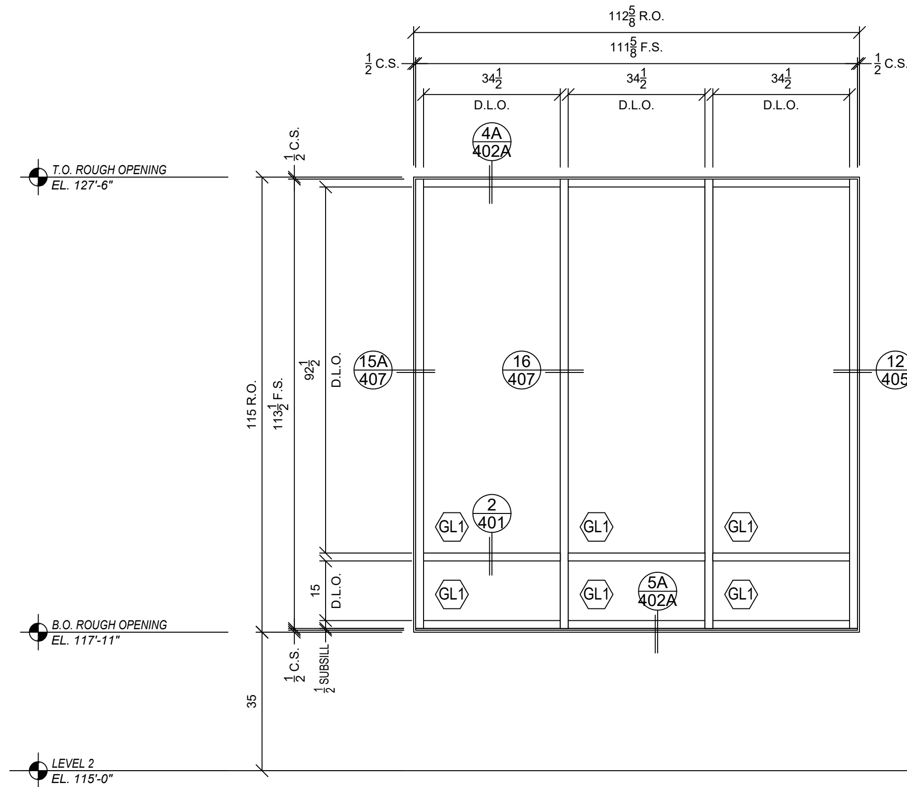
21 ELEVATION SF-13.1 ARCH REF: 2-A4.1.1, 2-A4.2.2 QTY: (1) TUBELITE T24650, 2" X 6.5", OUTSIDE GLAZED
