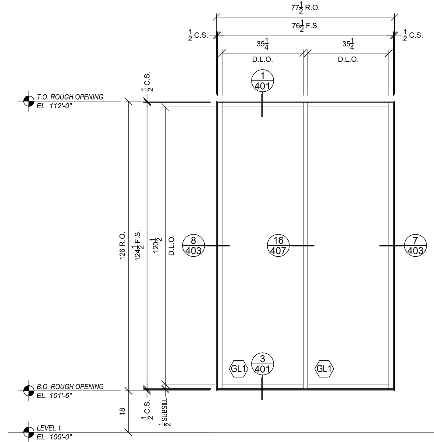
6 ELEVATION SF-3.2 ARCH REF: 2-A4.1.1, 2-A4.2.1 QTY: (1) TUBELITE T24650, 2" X 6.5", OUTSIDE GLAZED
