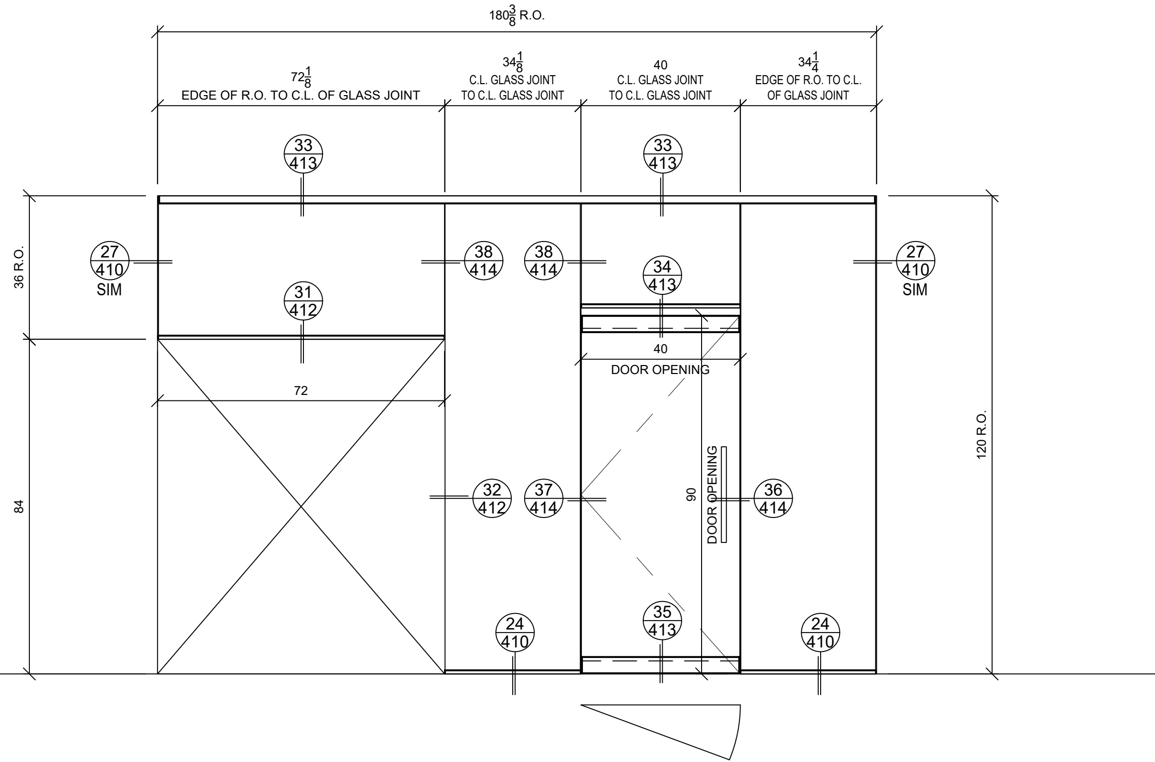
29 ELEVATION SF-25 ARCH REF: 20/2-A4.2.2 QTY: (1) 1" X 1" GLAZING CHANNEL
