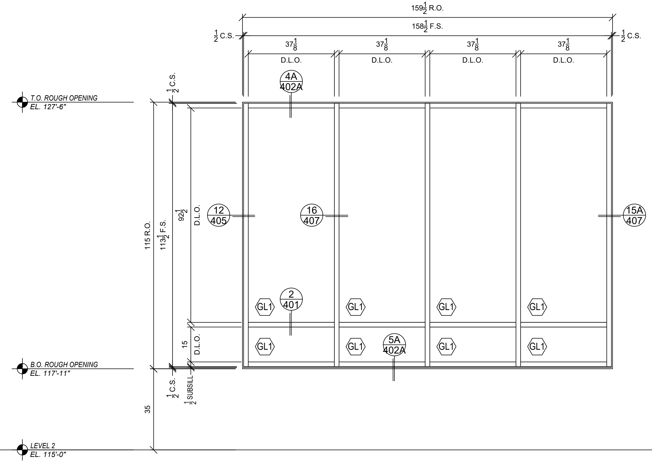
23 ELEVATION SF-13.3 ARCH REF: 2-A4.1.1, 2-A4.2.2 QTY: (1) TUBELITE T24650, 2" X 6.5", OUTSIDE GLAZED
